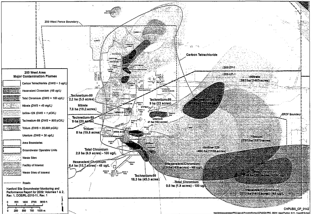
Figure 2. 200-UP-1 OU and 200-ZP-1 OU Groundwater Plume Map
